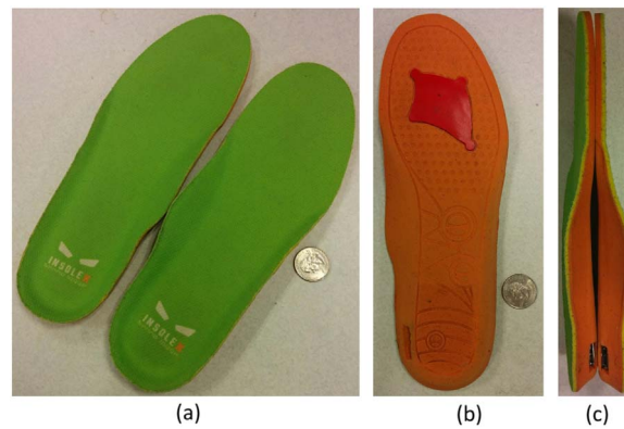
Fig. 1. The human ergonomic prototype of Smart Insole: (a) Front view; (b) Back view; (c) Lateral view.
